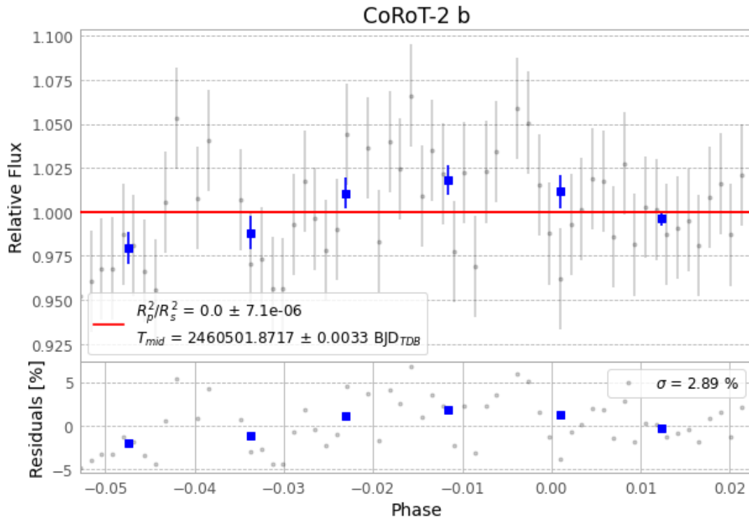
Figure 1 — FinalLightCurve_CoRoT-2 b_2024-07-09.png (SHA-256 b10b8cd002a4571b...)
