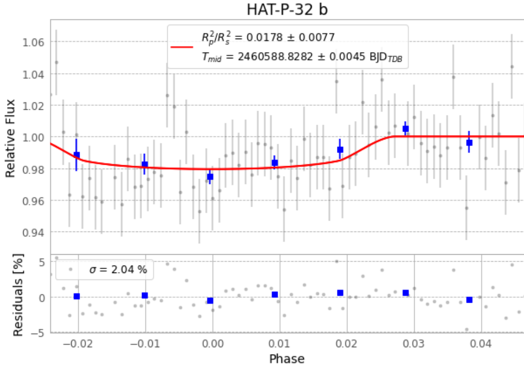
Figure 1 — FinalLightCurve_HAT-P-32 b_2024-10-04.png (SHA-256 df75828d08ebd1a1...)
