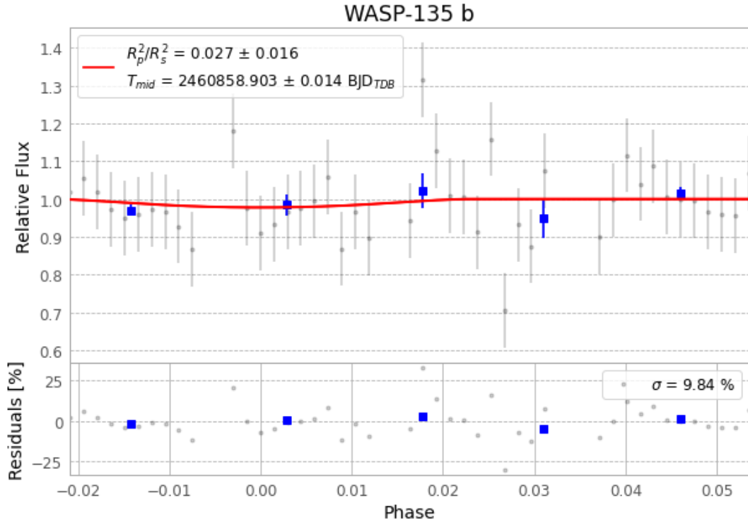
Figure 1 — FinalLightCurve_WASP-135 b_2025-07-02.png (SHA-256 24e2357a0b22298e...)
