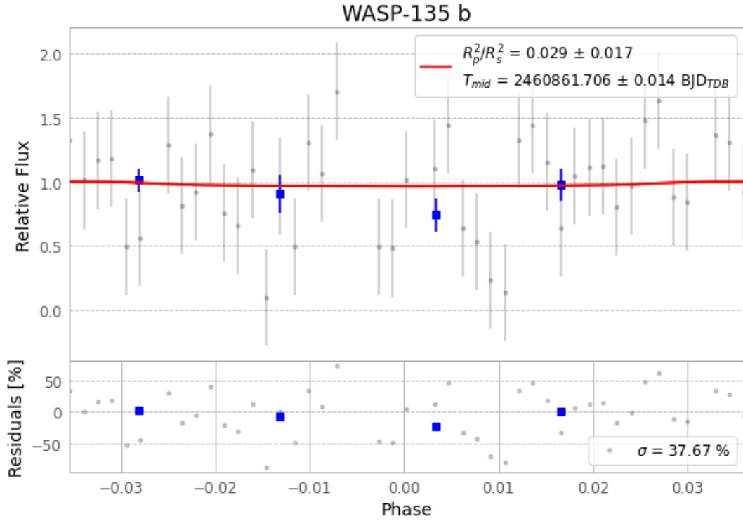
Figure 1 — FinalLightCurve_WASP-135 b_2025-07-04.png (SHA-256 d54264786d0cb814...)
