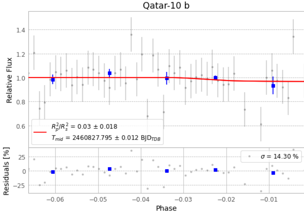
Figure 1 — FinalLightCurve_Qatar-10 b_2025-05-31.png (SHA-256 d3c91fed0aba9aa1...)
