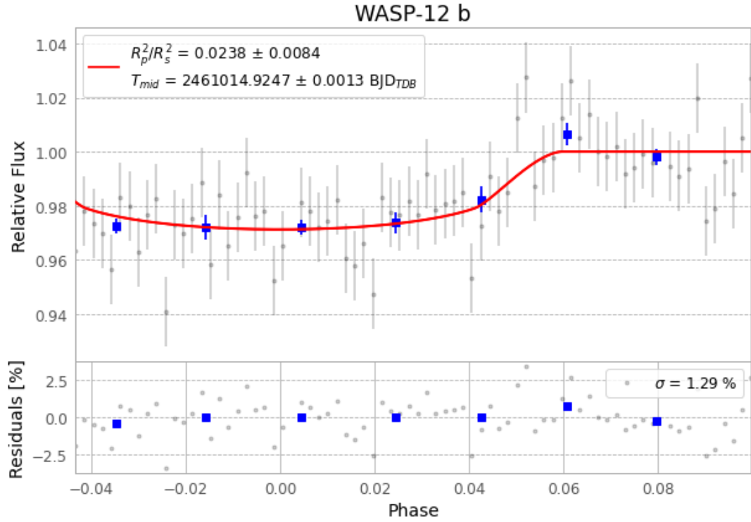
Figure 1 — FinalLightCurve_WASP-12 b_2025-12-05.png (SHA-256 a2bf50c5d1ede2cd...)
