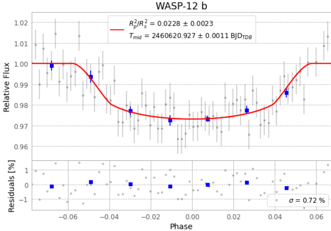
Figure 1 — FinalLightCurve_WASP-12 b_2024-11-06.png (SHA-256 0013767ecb9f6ee0...)
