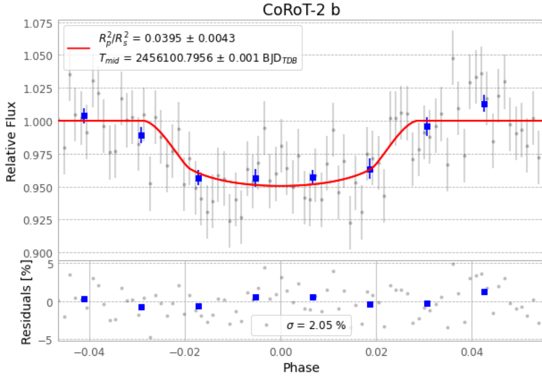
Figure 1 — FinalLightCurve_CoRoT-2 b_2012-06-21.png (SHA-256 89538affe57644b9...)
