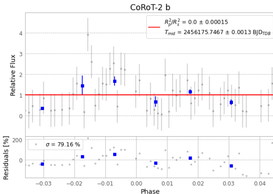
Figure 1 — FinalLightCurve_CoRoT-2 b_2012-09-04.png (SHA-256 24ff668b5607a74c...)
