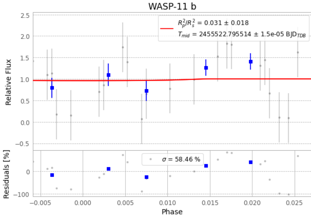
Figure 1 — FinalLightCurve_WASP-11 b_2010-11-21.png (SHA-256 2b516cf0253ffd86...)
