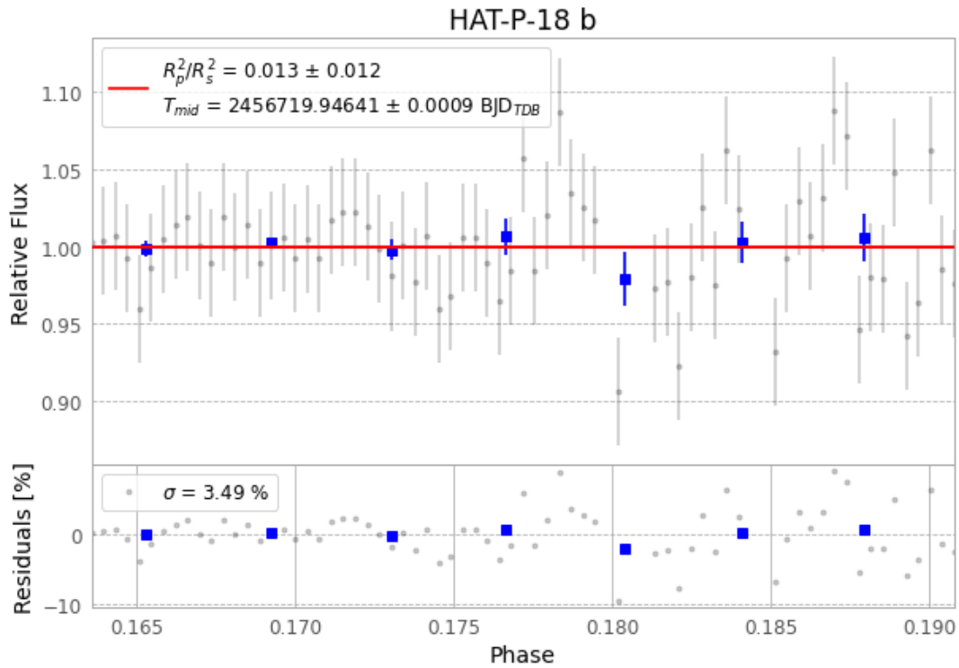
Figure 1 — FinalLightCurve_HAT-P-18 b_2014-03-04.png (SHA-256 3e5b9f352c82ff42...)
