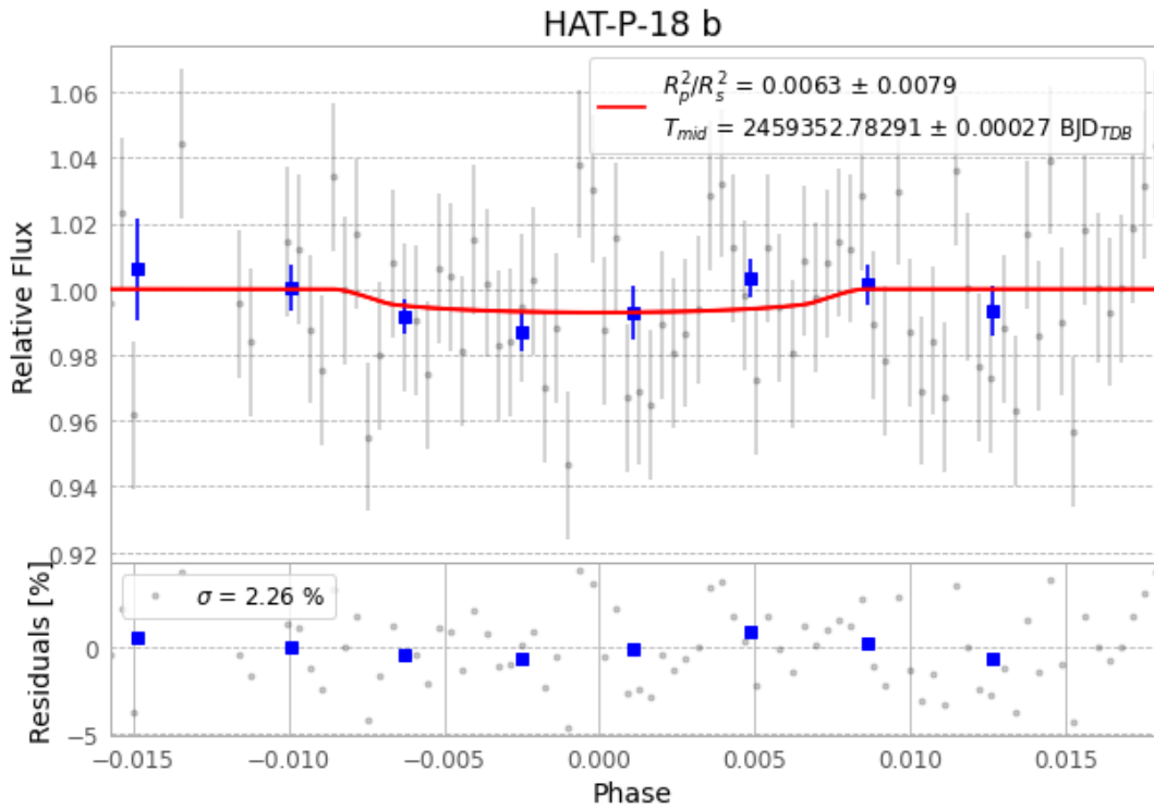
Figure 1 — FinalLightCurve_HAT-P-18 b_2021-05-17.png (SHA-256 6023055f1d5be803...)
