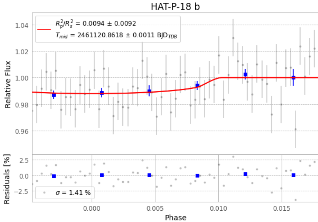
Figure 1 — FinalLightCurve_HAT-P-18 b_2026-03-21.png (SHA-256 393fe49b8f934bcc...)
