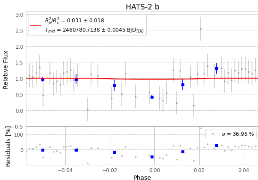
Figure 1 — FinalLightCurve_HATS-2 b_2025-04-14.png (SHA-256 a946e9d69262552...)
