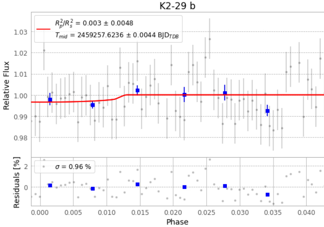
Figure 1 — FinalLightCurve_K2-29 b_2021-02-11.png (SHA-256 a20b49a5c89b58a8...)
