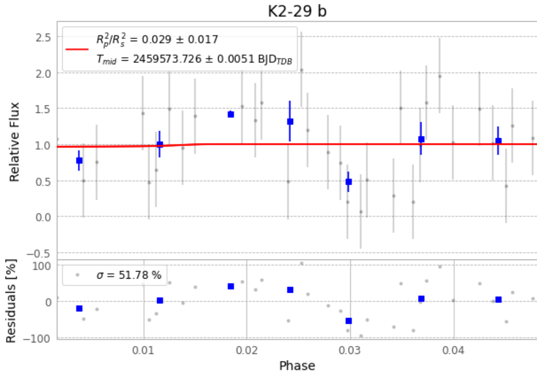
Figure 1 — FinalLightCurve_K2-29 b_2021-12-24.png (SHA-256 bd81689bb744947d...)
