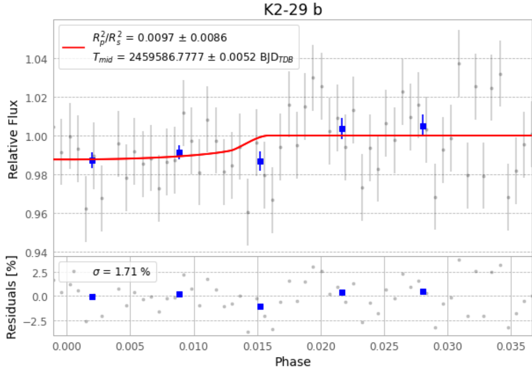
Figure 1 — FinalLightCurve_K2-29 b_2022-01-06.png (SHA-256 4867067bb7d33ba2...)
