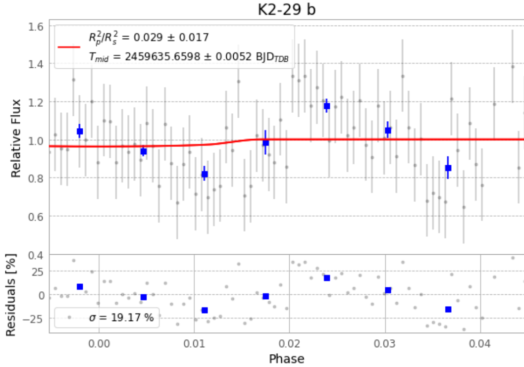
Figure 1 — FinalLightCurve_K2-29 b_2022-02-24.png (SHA-256 b952028289730304...)
