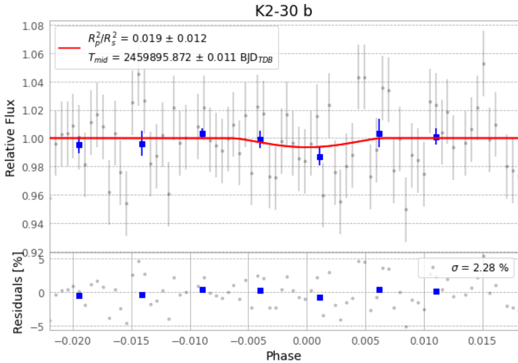
Figure 1 — FinalLightCurve_K2-30 b_2022-11-11.png (SHA-256 89289d81ccbc5f0...)
