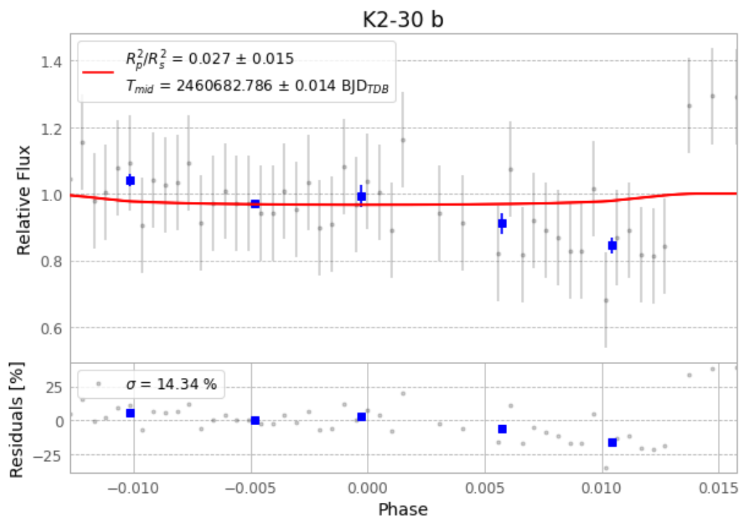
Figure 1 — FinalLightCurve_K2-30 b_2025-01-06.png (SHA-256 4155b9ef090d5f69...)
