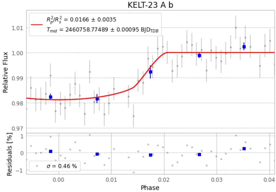
Figure 1 — FinalLightCurve_KELT-23 A b_2025-03-23.png (SHA-256 68bc6d0c37d4dc4f...)
