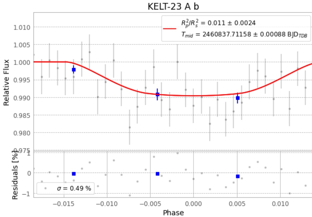
Figure 1 — FinalLightCurve_KELT-23 A b_2025-06-10.png (SHA-256 b7f64f778b02ddfc...)
