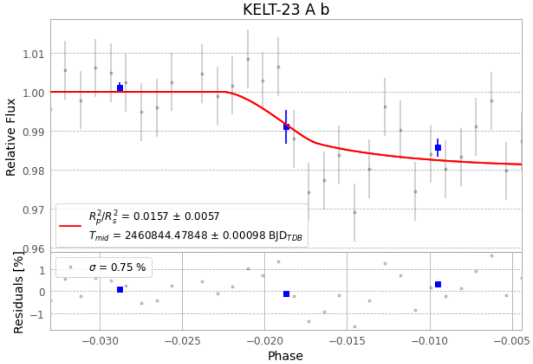
Figure 1 — FinalLightCurve_KELT-23 A b_2025-06-19.png (SHA-256 17c1f9f1e72b4d83...)
