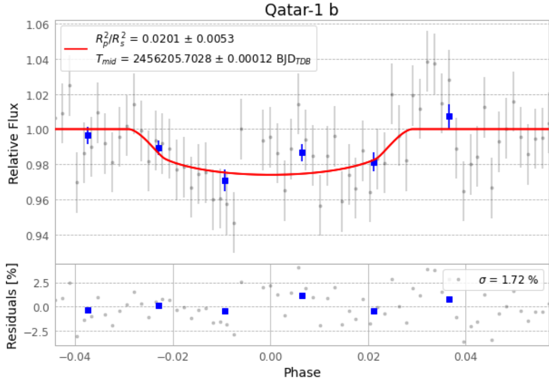
Figure 1 — FinalLightCurve_Qatar-1 b_2012-10-04.png (SHA-256 0b271e7f8d70082a...)
