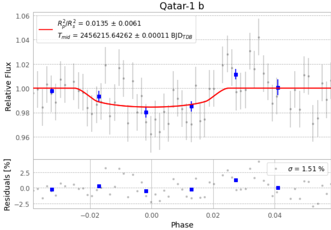
Figure 1 — FinalLightCurve_Qatar-1 b_2012-10-14.png (SHA-256 239661f4df81b9a0...)
