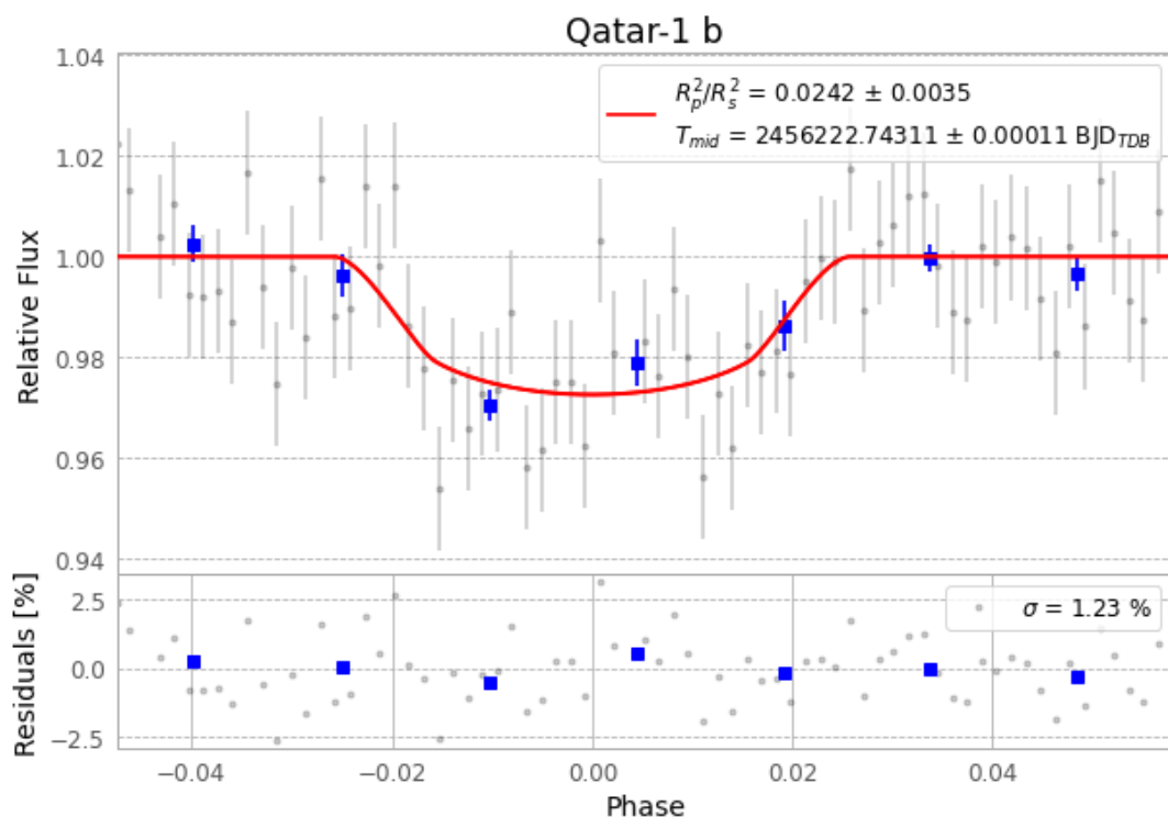
Figure 1 — FinalLightCurve_Qatar-1 b_2012-10-21.png (SHA-256 0f8aefb151740f1c...)
