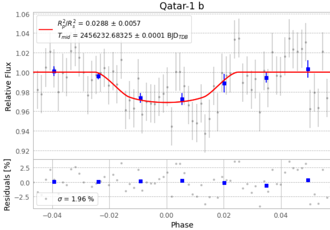
Figure 1 — FinalLightCurve_Qatar-1 b_2012-10-31.png (SHA-256 db1d3c6bfe184d4d...)
