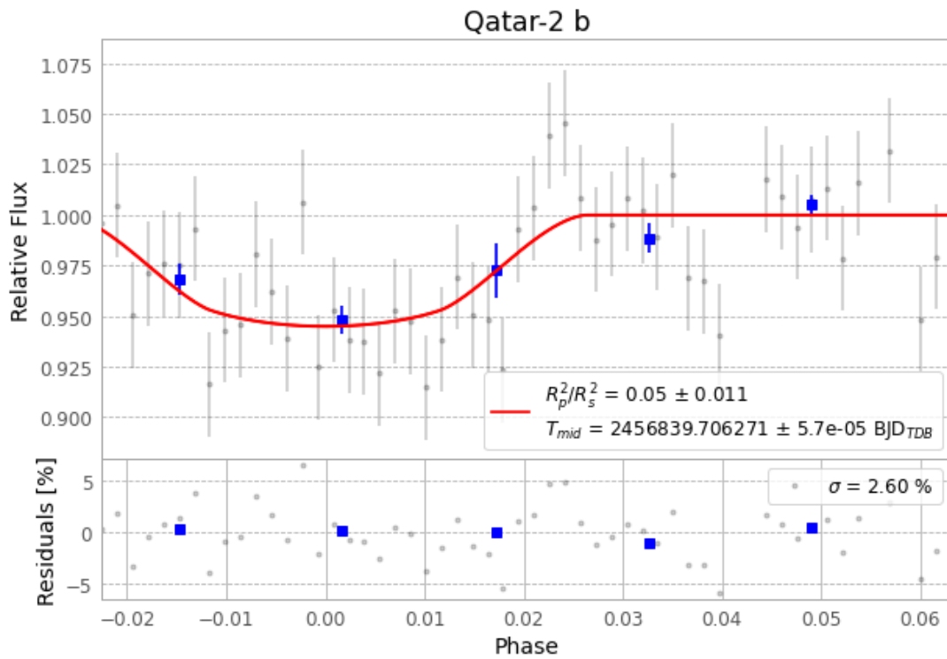
Figure 1 — FinalLightCurve_Qatar-2 b_2014-06-30.png (SHA-256 dc6e918006df82d1...)
