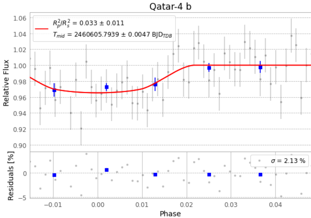
Figure 1 — FinalLightCurve_Qatar-4 b_2024-10-21.png (SHA-256 5926aabdb4efd21f...)
