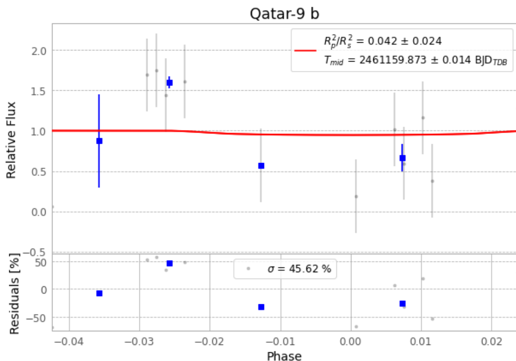
Figure 1 — FinalLightCurve_Qatar-9 b_2026-04-29.png (SHA-256 5325f72636e562d5...)
