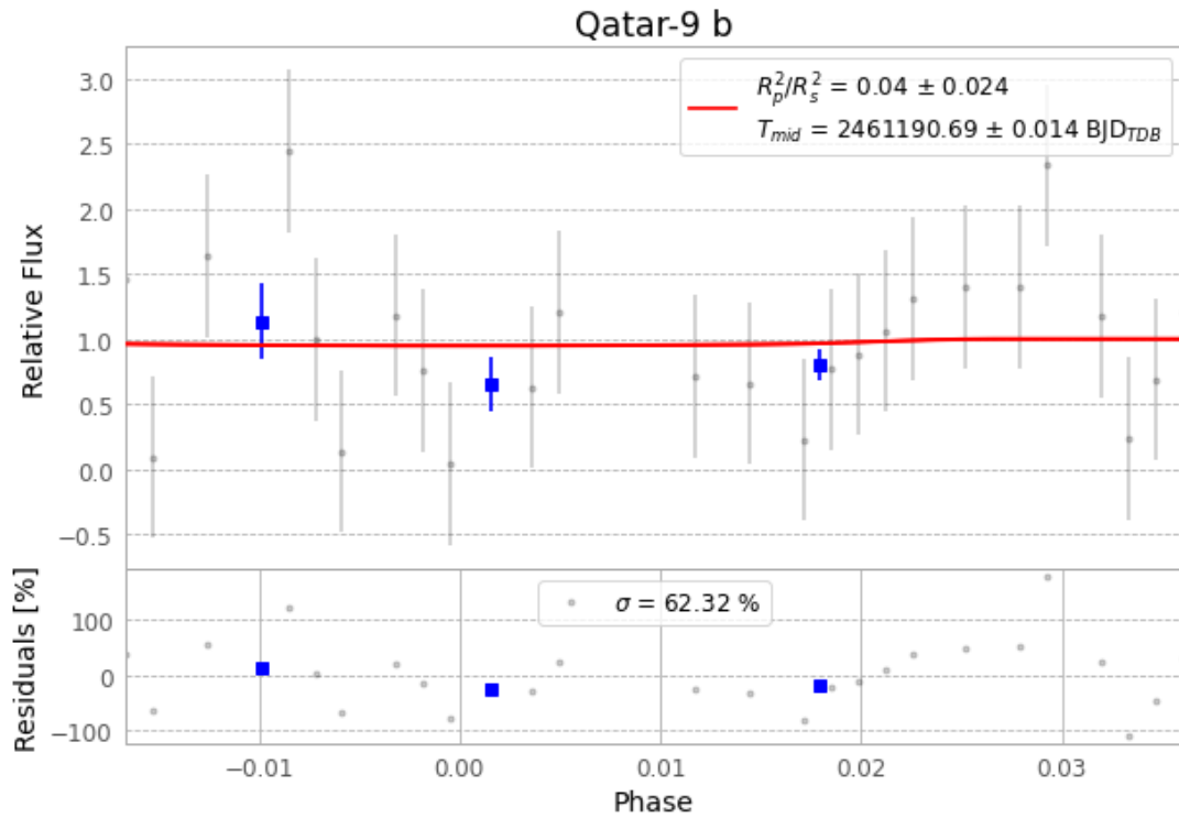
Figure 1 — FinalLightCurve_Qatar-9 b_2026-05-29.png (SHA-256 56dac940fa4a6136...)
