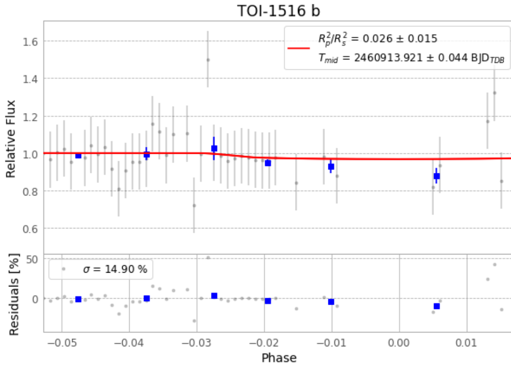
Figure 1 — FinalLightCurve_TOI-1516 b_2025-08-26.png (SHA-256 13124438b08f4cb1...)
