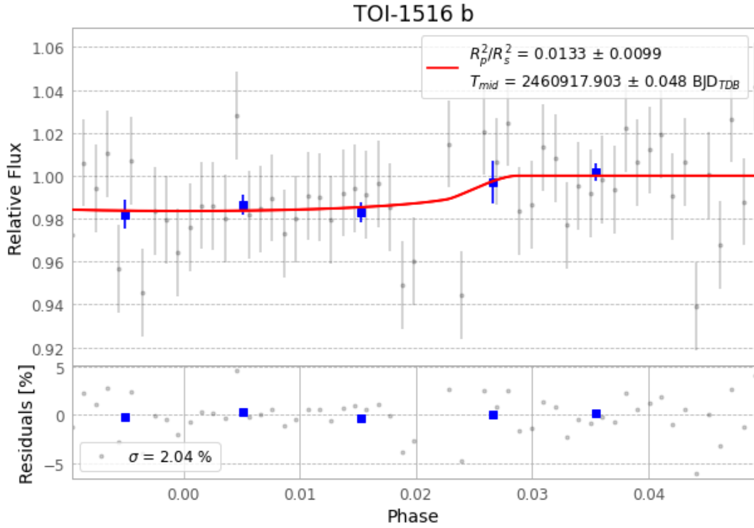
Figure 1 — FinalLightCurve_TOI-1516 b_2025-08-30.png (SHA-256 a82cb767aff8f30d...)
