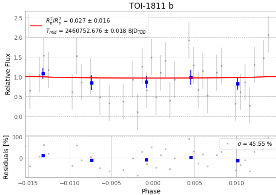
Figure 1 — FinalLightCurve_TOI-1811 b_2025-03-17.png (SHA-256 eefa79678e556066...)
