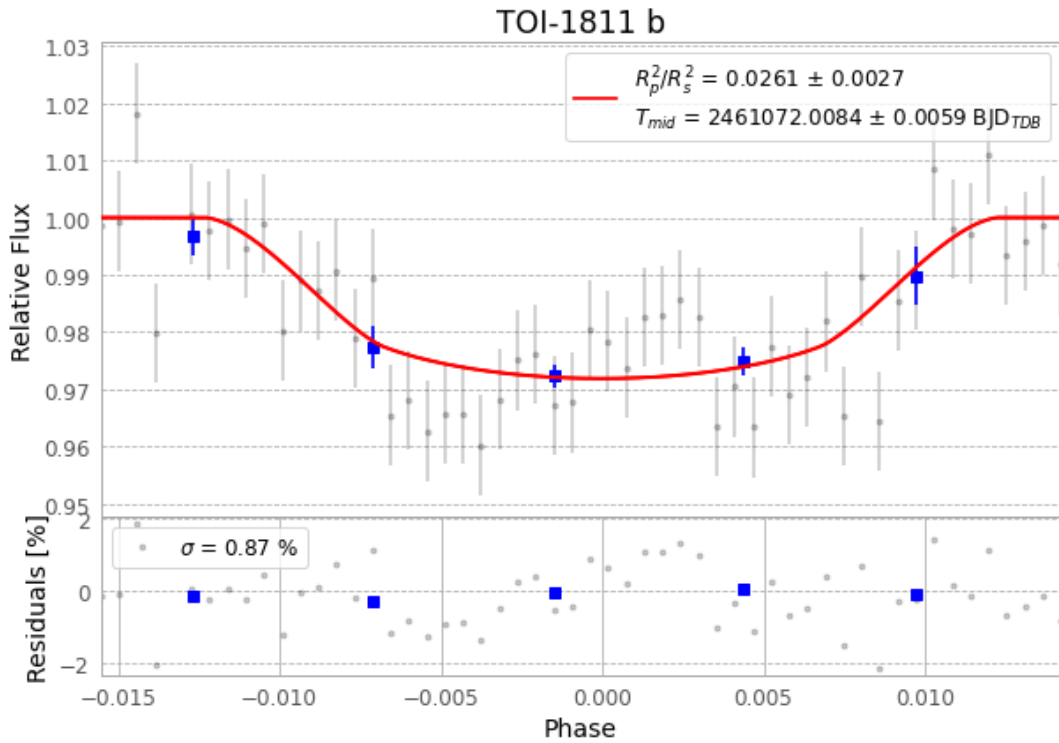
Figure 1 — FinalLightCurve_TOI-1811 b_2026-01-31.png (SHA-256 cd76f7cb08cfa67f...)
