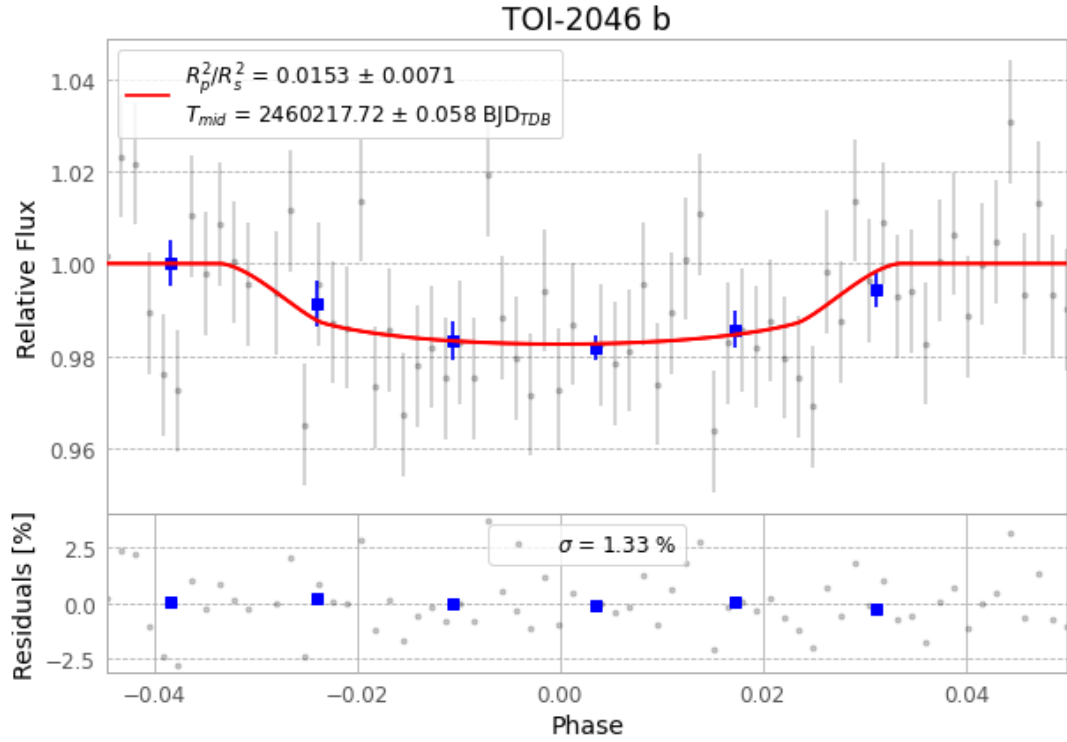
Figure 1 — FinalLightCurve_TOI-2046 b_2023-09-29.png (SHA-256 150119fc90bc5393...)
