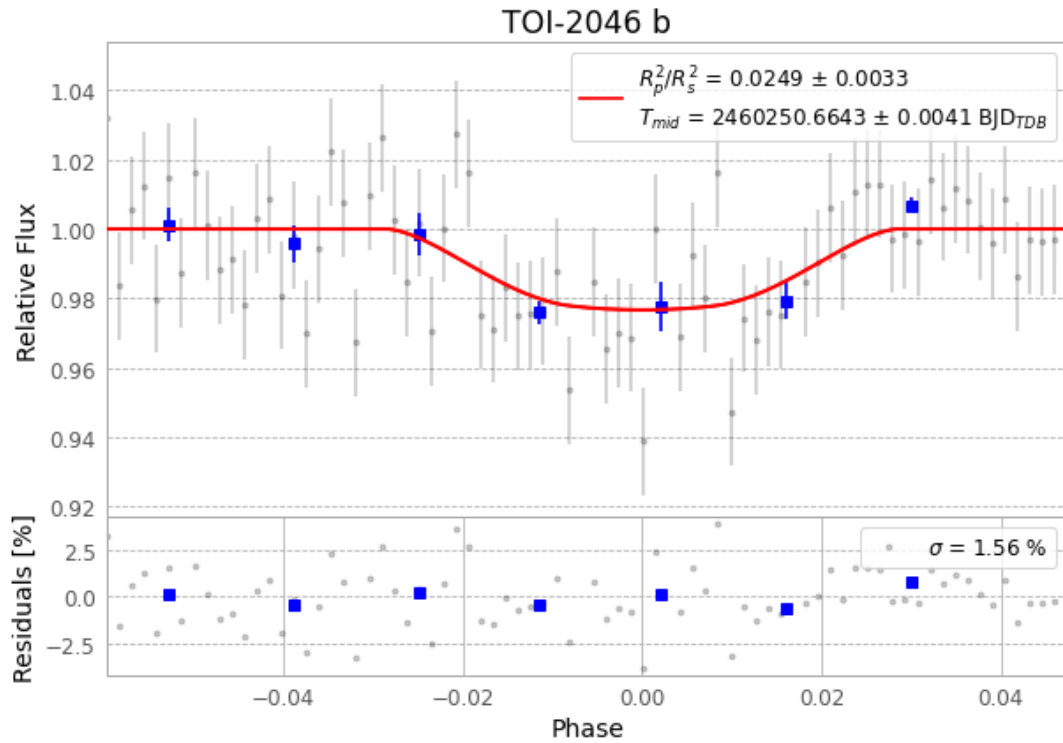
Figure 1 — FinalLightCurve_TOI-2046 b_2023-11-01.png (SHA-256 8da7c75eb1a0b7d6...)
