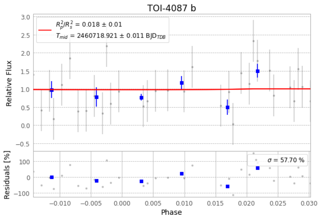
Figure 1 — FinalLightCurve_TOI-4087 b_2025-02-12.png (SHA-256 57eedede2cbd1207...)
