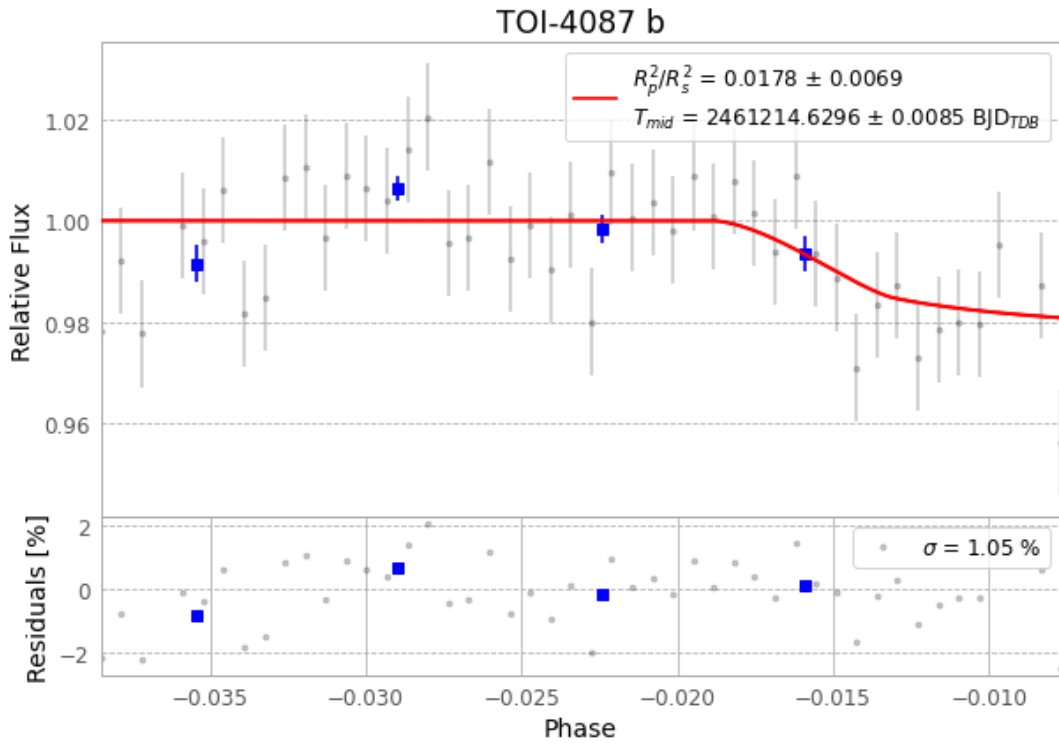
Figure 1 — FinalLightCurve_TOI-4087_b_2026-06-25.png (SHA-256 fcf5daab41102a5d...)
