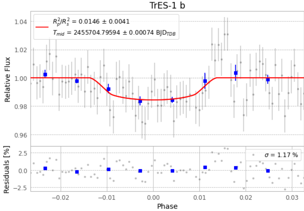
Figure 1 — FinalLightCurve_TrES-1 b_2011-05-22.png (SHA-256 da0a0f3a9c8a8dc2...)
