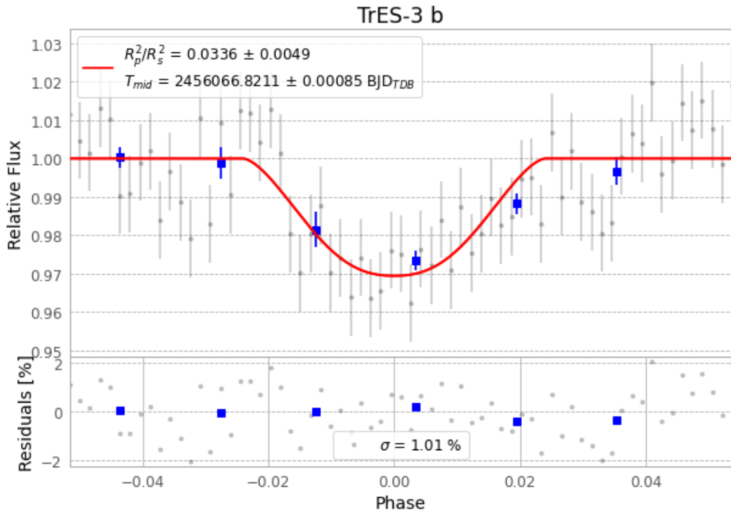
Figure 1 — FinalLightCurve_TrES-3 b_2012-05-18.png (SHA-256 f403053b0891f524...)
