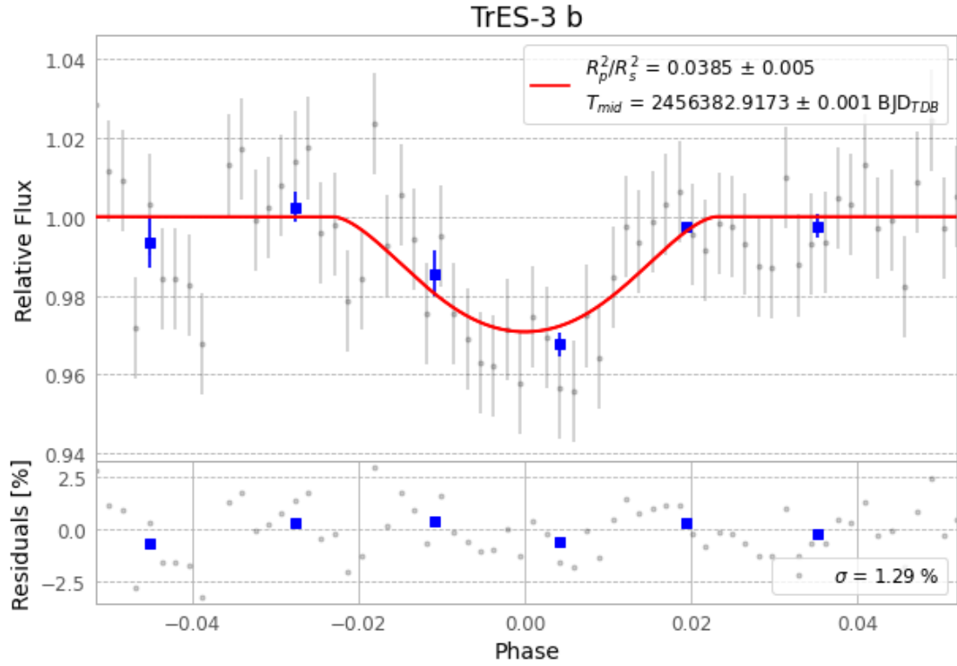
Figure 1 — FinalLightCurve_TrES-3 b_2013-03-31.png (SHA-256 030a30ef3259c6f3...)
