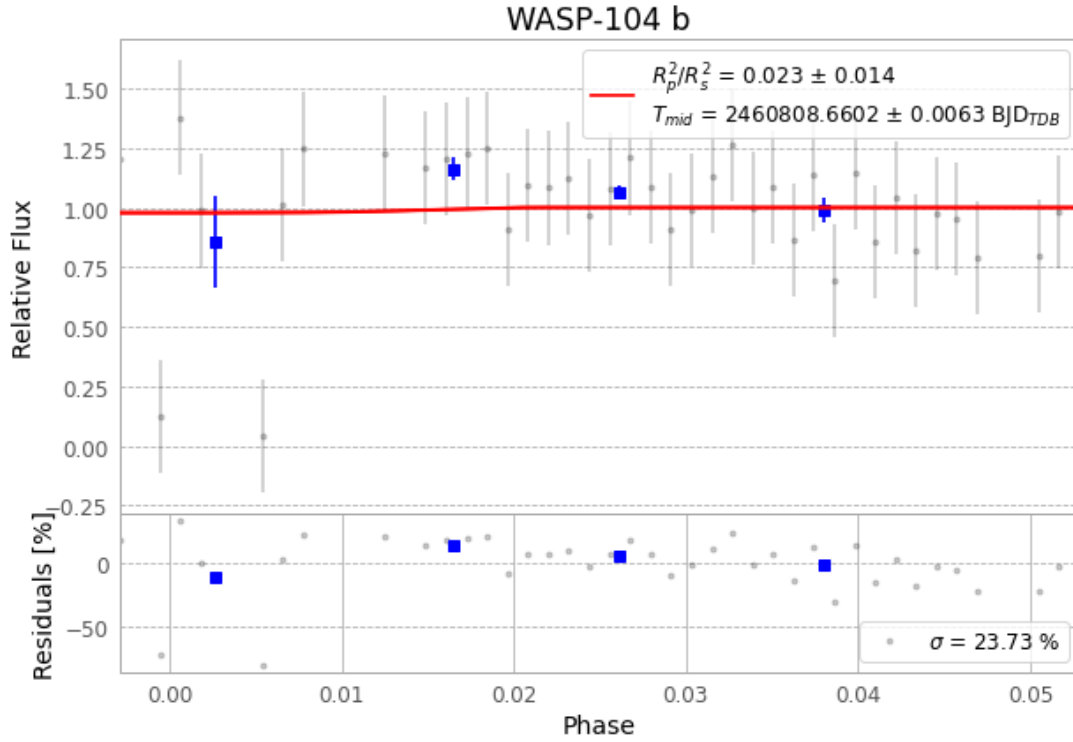
Figure 1 — FinalLightCurve_WASP-104 b_2025-05-12.png (SHA-256 99a06a9674798f54...)
