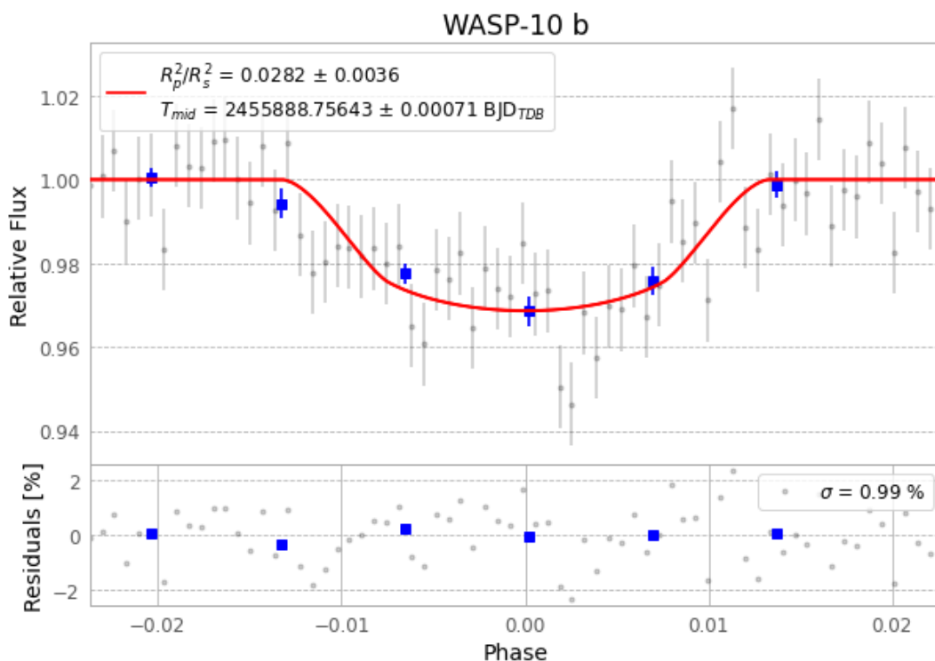
Figure 1 — FinalLightCurve_WASP-10 b_2011-11-22.png (SHA-256 036ea7db229a8a54...)
