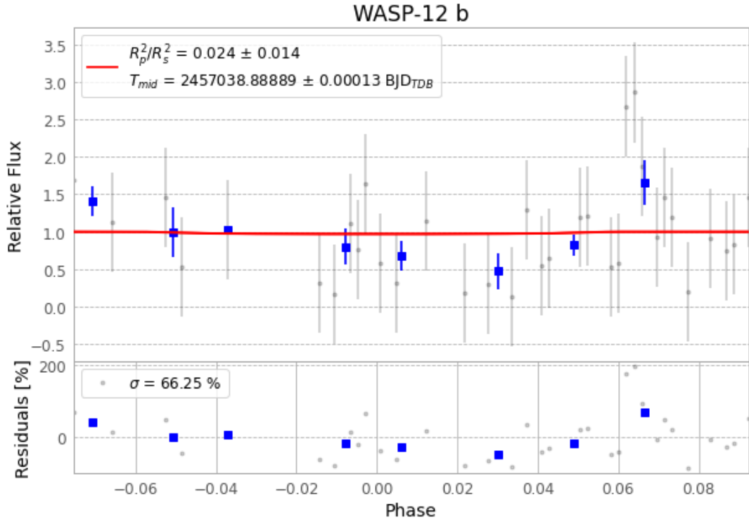
Figure 1 — FinalLightCurve_WASP-12 b_2015-01-16.png (SHA-256 202a5bebf01ca410...)
