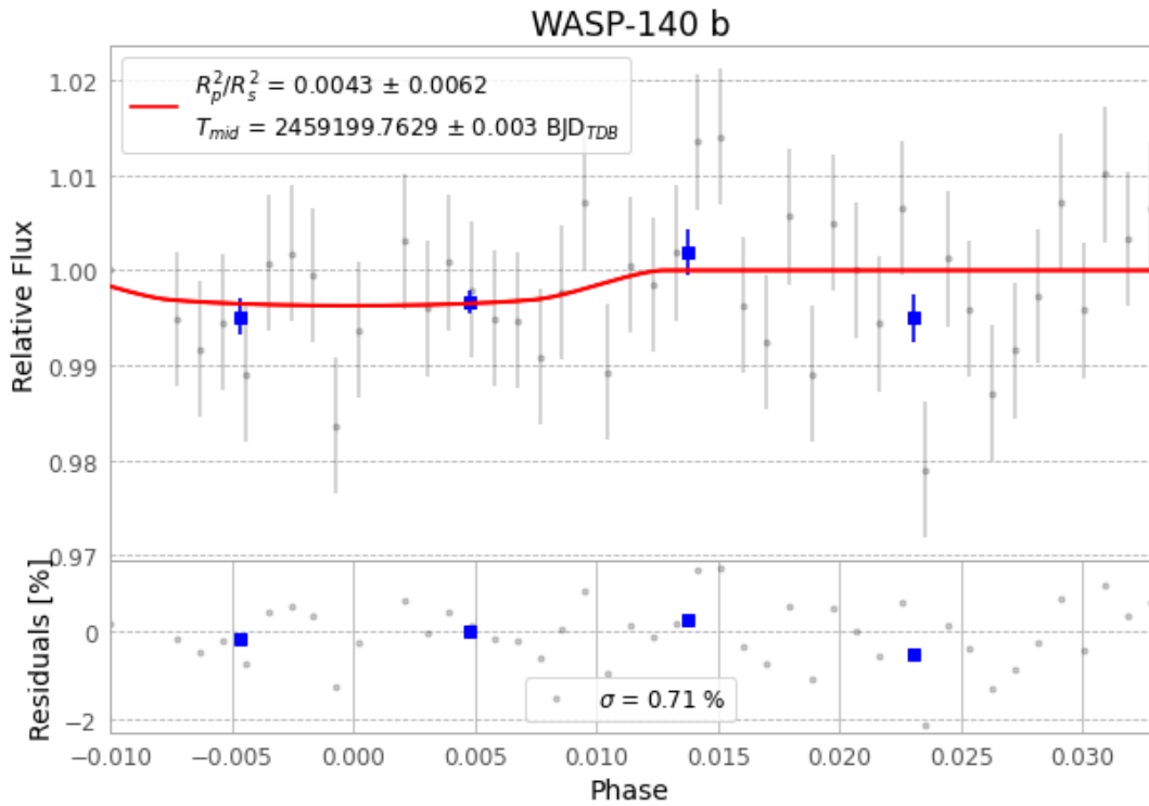
Figure 1 — FinalLightCurve_WASP-140 b_2020-12-15.png (SHA-256 6a4ab5cd976788e7...)
