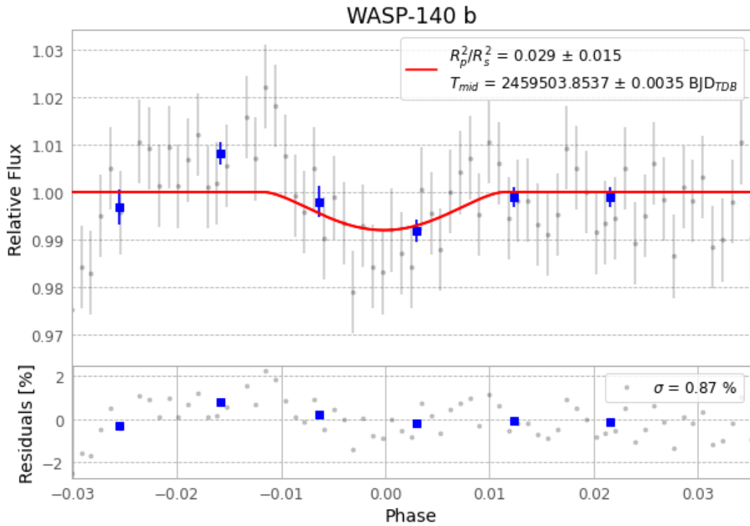
Figure 1 — FinalLightCurve_WASP-140 b_2021-10-15.png (SHA-256 ccf3b75bb3afa265...)
