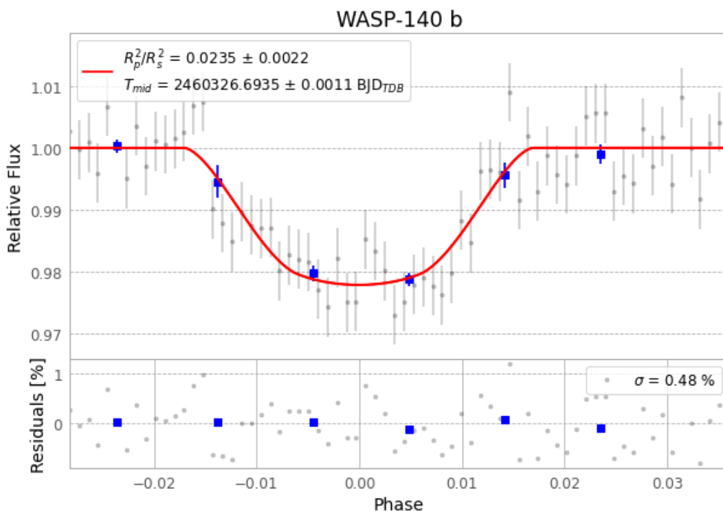
Figure 1 — FinalLightCurve_WASP-140 b_2024-01-16.png (SHA-256 ff3fb7cc474706f4...)
