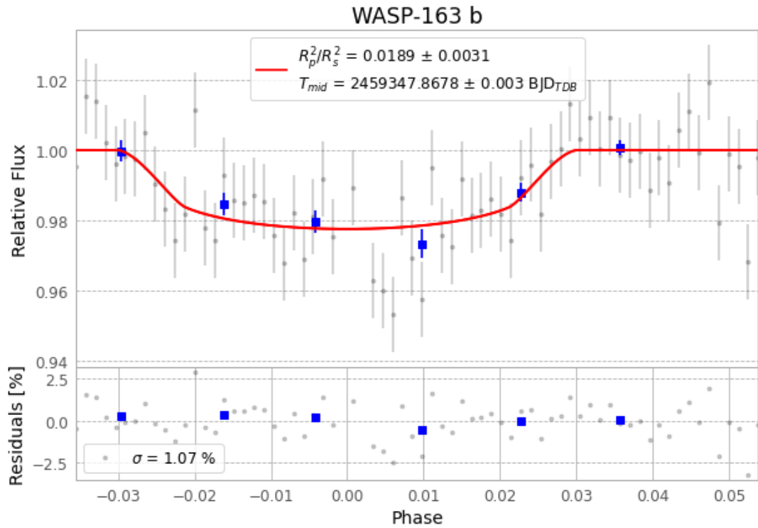
Figure 1 — FinalLightCurve_WASP-163 b_2021-05-13.png (SHA-256 cce27d15c5381663...)
