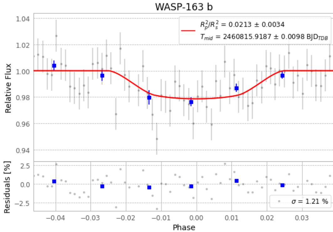
Figure 1 — FinalLightCurve_WASP-163 b_2025-05-20.png (SHA-256 7f76b1d71e5acde3...)
